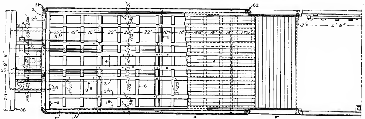
Fig. 578. Part Plan of Underframing.
